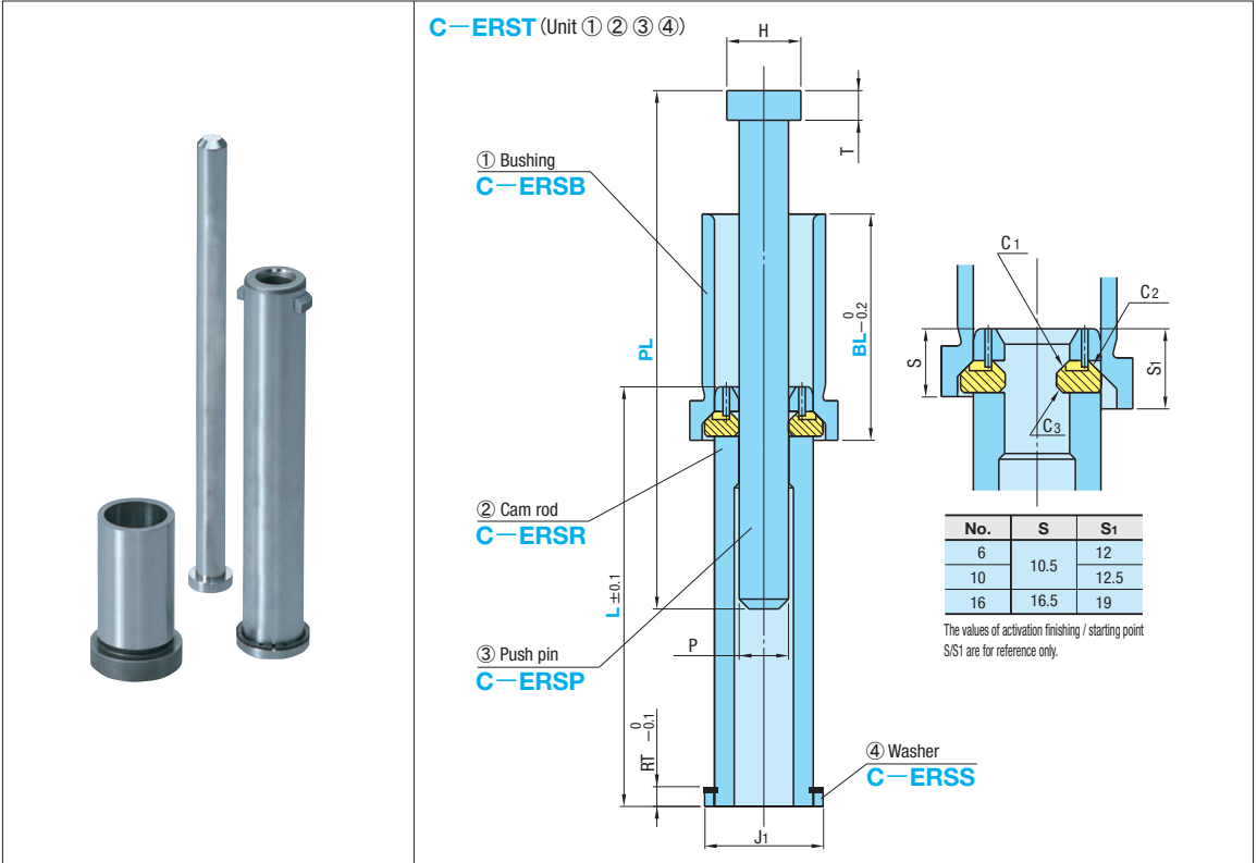
① Bushing C-ERSB
