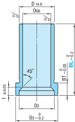
① Bushing C-ERSB
