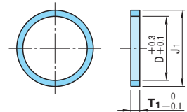
④ Washer C-ERSS
